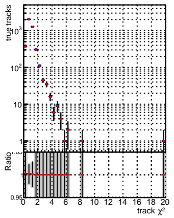
2 of associated (recoToSim) tracks vs normalized \chi^2
