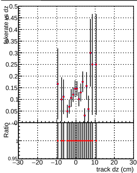
—•— DQM_V0001_R0000000001_Global_mkFit100PIXLLNO_RECO —•— DQM_V0001_R0000000001_Global_mkFit100PIXLL_RECO
