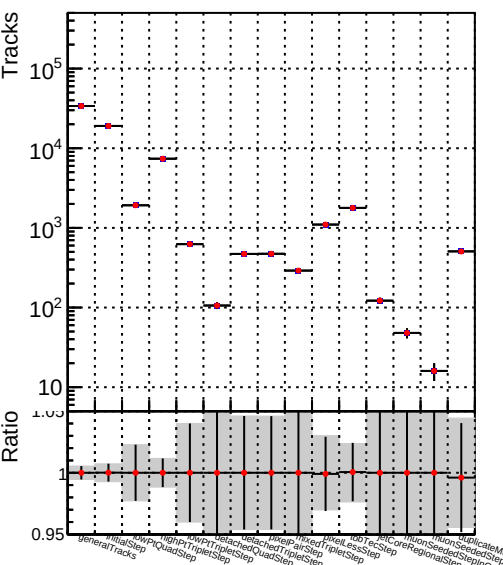
DQM_V0001_R000000001_Global_mkFit100PIXLLNO_RECO
