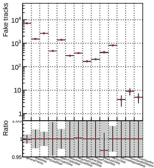
Number ● DQM_V0001_R000000001_Global_mkFit100PIXLL_RECO
