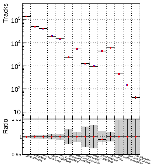
DQM_V0001_R000000001__Global__mkFit100PIXLLNO__RECO
