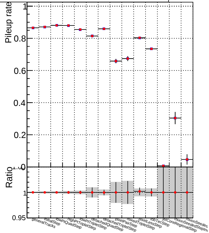
DQM_V0001_R000000001_Global_mkFit100PIXLLNO_RECO
