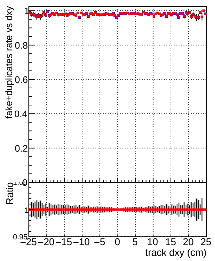
DQM_V0001_R000000001_Global_mkFit100PIXLLNO_RECO DQM_V0001_R000000001_Global_mkFit100PIXLL_RECO
