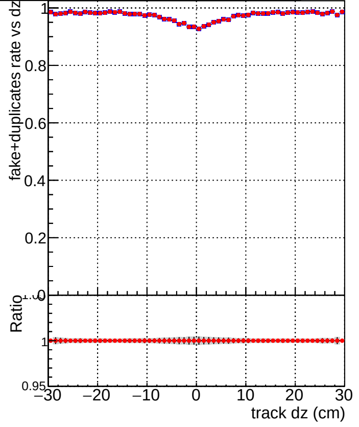
DQM_V0001_R000000001_Global_mkFit100PIXLLNO_RECO DQM_V0001_R000000001_Global_mkFit100PIXLL_RECO
