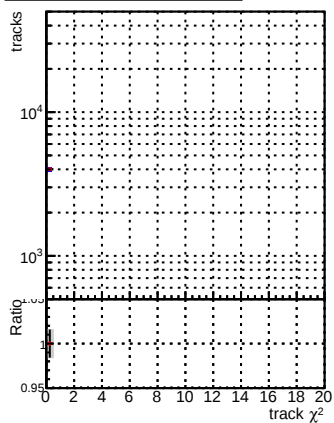
N of reco track vs. \chi^2 for DQM_V0001_R0000000001_Global_mkFit100PIXLLNO_RECO (blue) and DQM_V0001_R0000000001_Global_mkFit100PIXLL_RECO (red)
