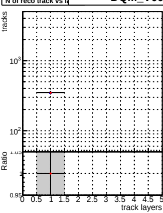
N of reco track vs track layer
