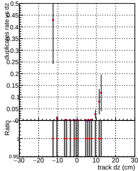
Fake rate vs dz DQM_V0001_R0000000001_Global_mkFit100PIXLLNO_RECO Duplicates rate vs dz DQM_V0001_R0000000001_Global_mkFit100PIXLL_RECO
