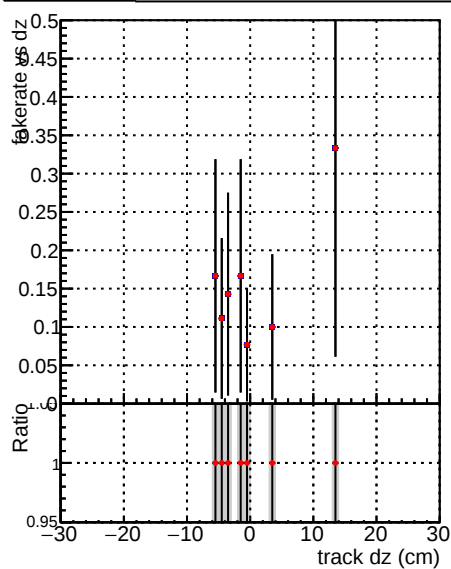
Fake rate vs d Legend: DQM_V0001_R000000001_Global_mkFit100PIXLLNO_RECO DQM_V0001_R000000001_Global_mkFit100PIXLL_RECO
