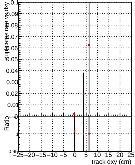
—●— DQM_V0001_R0000000001_Global_mkFit100PIXLLNO_RECO —●— DQM_V0001_R0000000001_Global_mkFit100PIXLL_RECO
