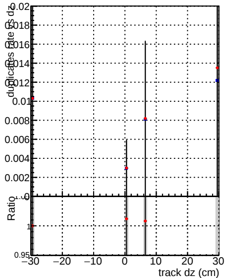
—●— DQM_V0001_R0000000001_Global_mkFit100PIXLLNO_RECO —●— DQM_V0001_R0000000001_Global_mkFit100PIXLL_RECO
