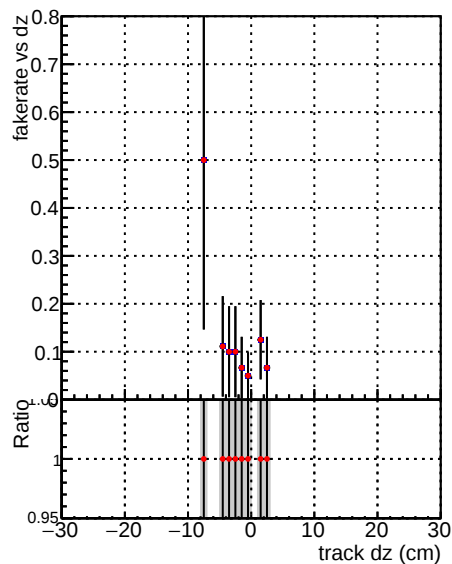
█ █ DQM_V0001_R0000000001 Global mkFit100PIXLLNO RECO █ █ DQM_V0001_R0000000001 Global mkFit100PIXLL RECO
