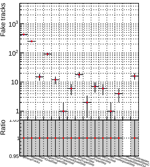
Number —●— DQM_V0001_R000000001_Global_mkFit100PIXLL_RECO
