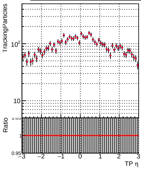
N of simulated tracks vs \eta Legend: DQM_V0001_R000000001_Global_mkFit100PIXLLNO_RECO (blue line), DQM_V0001_R000000001_Global_mkFit100PIXLL_RECO (red line)
