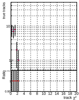
N of reco track vs. \chi^2 — Global_mkFit100PIXLLN_RECO — Global_mkFit100PIXLL_RECO
