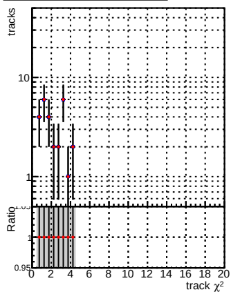
N of reco track vs. \chi^2 for DQM V0001_R000000001_Global_mkFit100PIXLLNO_RECO (blue) and DQM V0001_R000000001_Global_mkFit100PIXLL_RECO (red)
