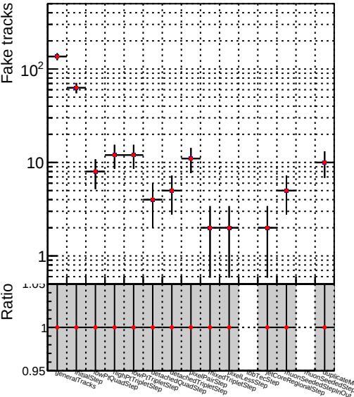
Number —●— DQM_V0001_R000000001_Global_mkFit100PIXLL_RECO
