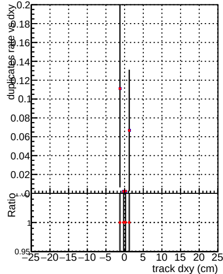
al_mkFit100PIXLL RECO
