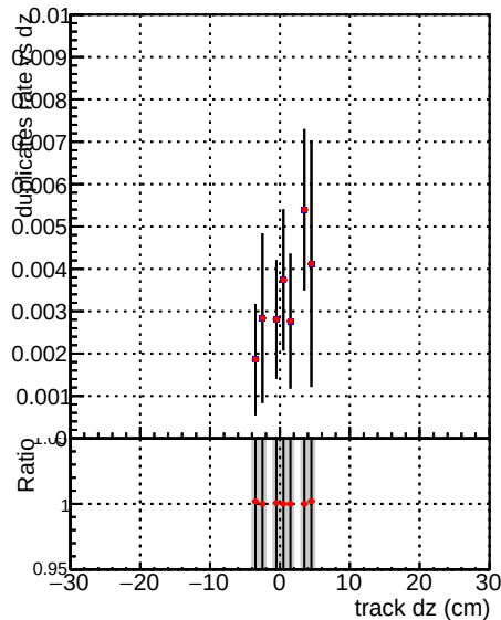
al_mkFit100PIXLL RECO
