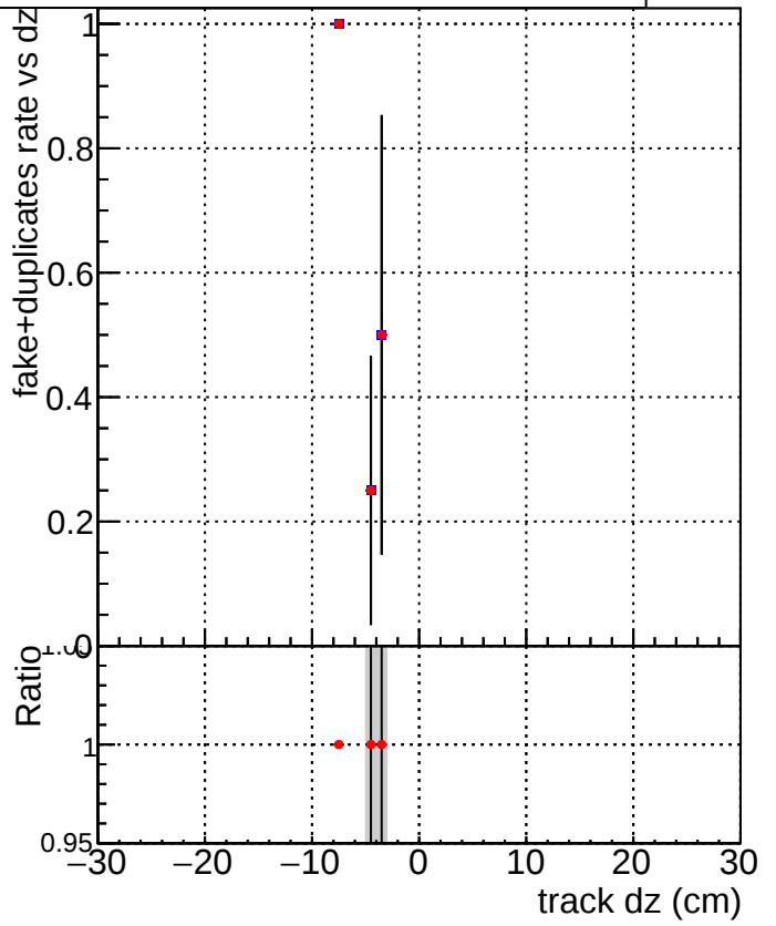
DQM_V0001_R000000001_Global_mkFit100PIXLLNO_RECO DQM_V0001_R000000001_Global_mkFit100PIXLL_RECO
