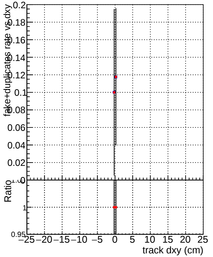
DQM_V0001_R000000001_Global_mkFit100PIXLLNO_RECO DQM_V0001_R000000001_Global_mkFit100PIXLL_RECO
