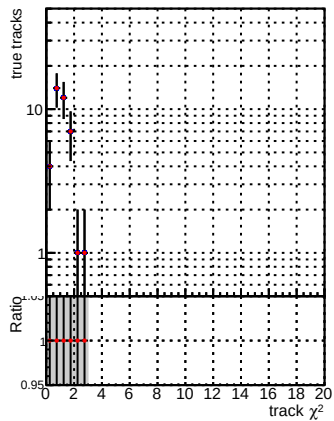
N of reco track vs. \chi^2 — Global_mkFit100PIXLLNO_RECO — Global_mkFit100PIXLL_RECO
