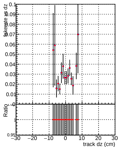
Fake rate vs dz —•— DQM_V0001_R0000000001_Global_mkFit100PIXLLNO_RECO —•— DQM_V0001_R0000000001_Global_mkFit100PIXLL_RECO
