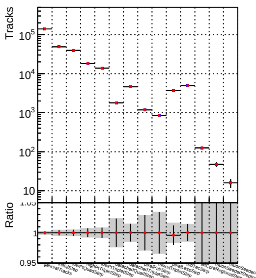
DQM_V0001_R000000001_Global_mkFit100PIXLLNO_RECO
