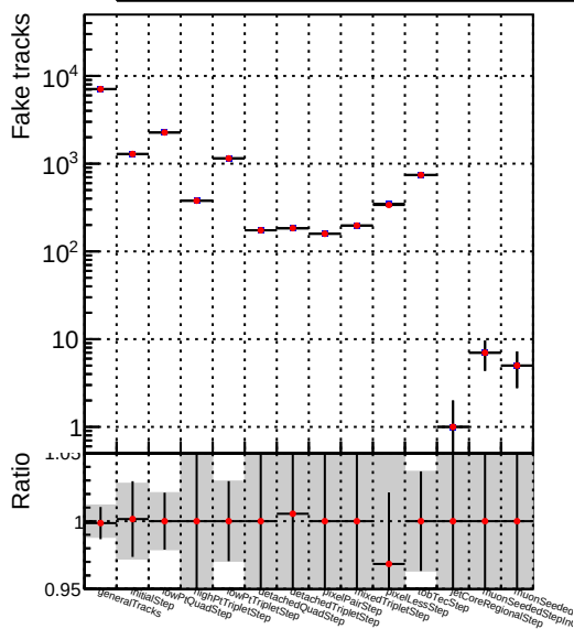
Number ● DQM_V0001_R000000001_Global_mkFit100PIXLL_RECO
