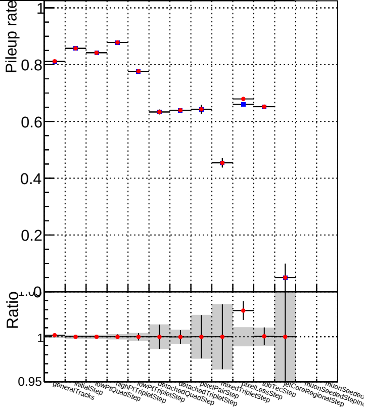
DQM_V0001_R000000001_Global_mkFit100PIXLLNO_RECO
