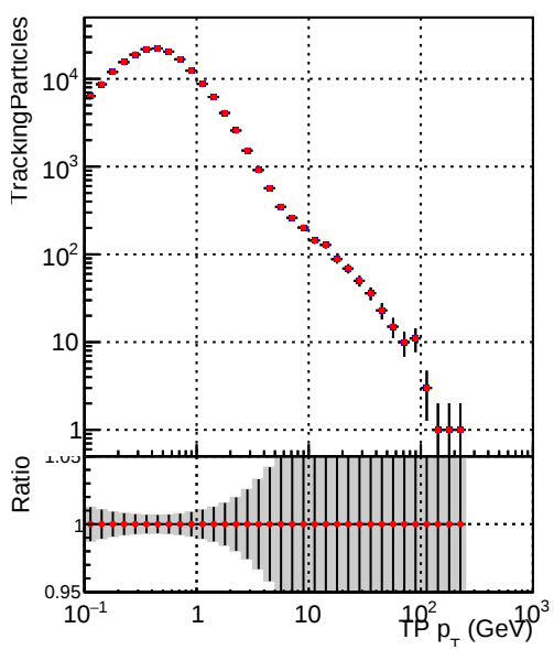
—●— DQM_V0001_R0000000001_Global_mkFit100PIXLLNO_RECO —●— DQM_V0001_R0000000001_Global_mkFit100PIXLL_RECO
