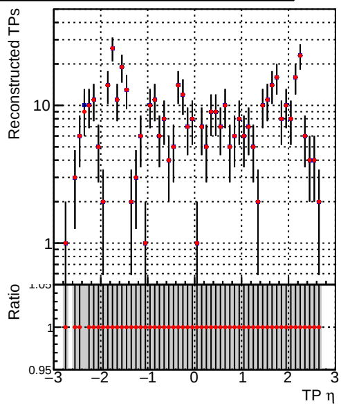
—●— DQM_V0001_R0000000001_Global_mkFit100PIXLLNO_RECO —●— DQM_V0001_R0000000001_Global_mkFit100PIXLL_RECO
