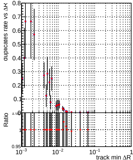
—●— DQM_V0001_R000000001_Global_mkFit100PIXLLNO_RECO —●— DQM_V0001_R000000001_Global_mkFit100PIXLL_RECO
