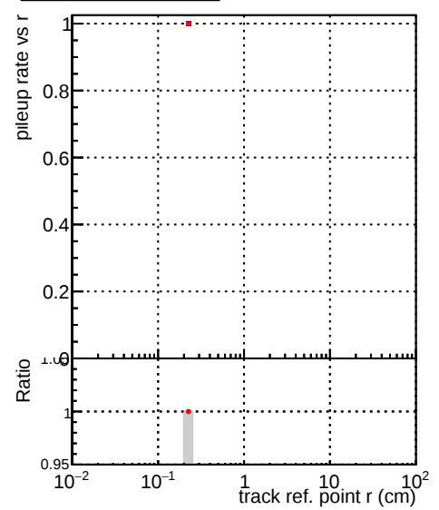
DQM_V0001_R000000001_Global_mkFit100PIXLLNO_RECO DQM_V0001_R000000001_Global_mkFit100PIXLL_RECO
