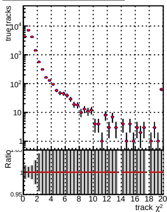
1 Global mkFit100PIXLLNO RECO 1 Global mkFit100PIXLL RECO
