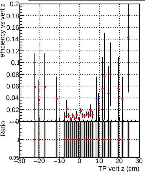
Efficiency vs vertpos Legend: DQM_V0001_R000000001_Global_mkFit100PIXLLNO_RECO DQM_V0001_R000000001_Global_mkFit100PIXLL_RECO
