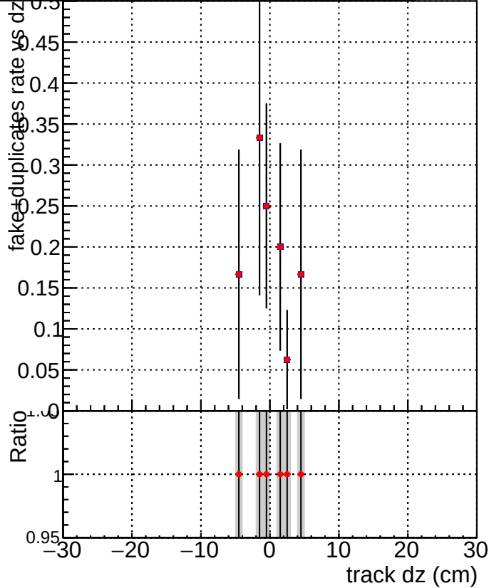
DQM_V0001_R000000001_Global_mkFit100PIXLLNO_RECO DQM_V0001_R000000001_Global_mkFit100PIXLL_RECO
