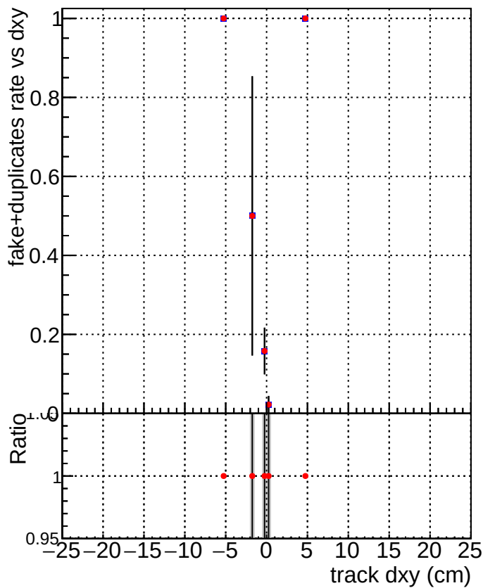
DQM_V0001_R000000001_Global_mkFit100PIXLLNO_RECO DQM_V0001_R000000001_Global_mkFit100PIXLL_RECO
