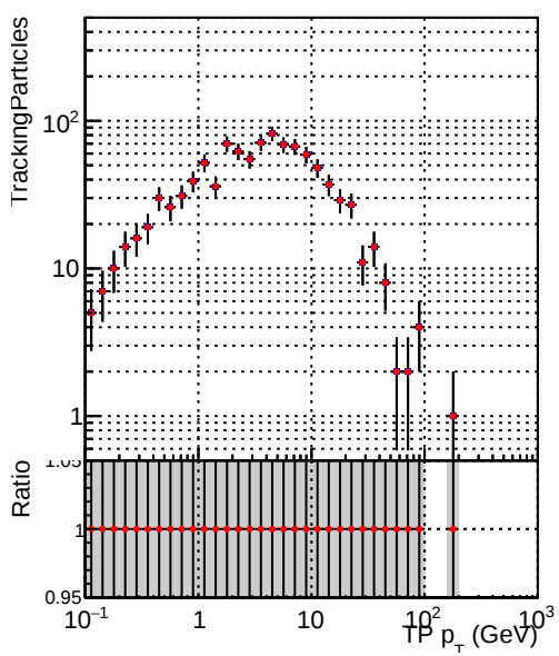
Legend: — DQM_V0001_R0000000001_Global_mkFit100PIXLLNO_RECO — DQM_V0001_R0000000001_Global_mkFit100PIXLL_RECO
