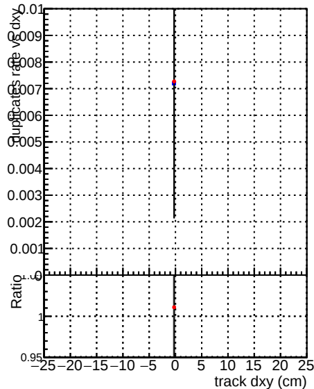
—●— DQM_V0001_R0000000001_Global_mkFit100PIXLLNO_RECO —●— DQM_V0001_R0000000001_Global_mkFit100PIXLL_RECO
