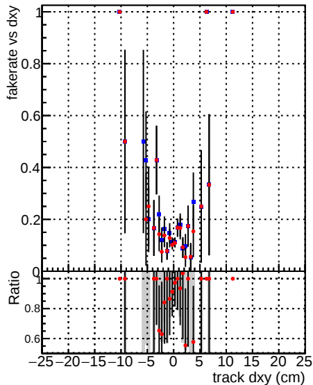
—●— DQM_V0001_R0000000001_Global_mkFit100PIXLLNO_RECO —●— DQM_V0001_R0000000001_Global_mkFit100PIXLL_RECO
