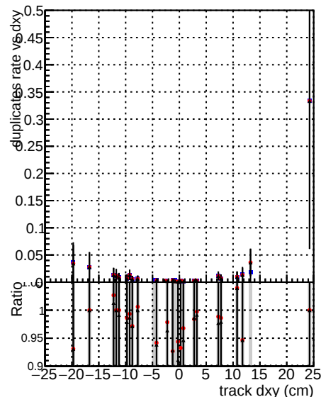
Legend for Fake rate vs dxy, Duplicates Rate vs Dxy, and Pileup rate vs dxy plots: DOM V0001 R0000000001 Global mkFit baseline DOM V0001 R0000000001 Global mkFit [core]maxCand-24DUPremoval-1000
