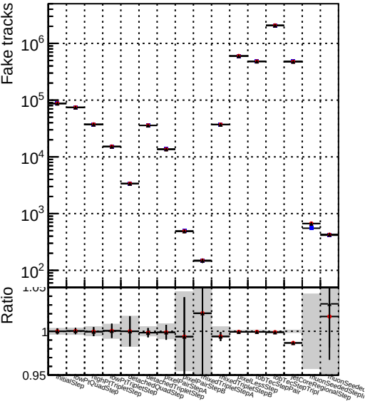
Number Configuration 1 DQM_V0001_R0000000001_Global_mkFit_jcore50maxCand-24DUPremoval-1000 2 DQM_V0001_R0000000001_Global_mkFit_jcore10maxCand-24DUPremoval-1000
