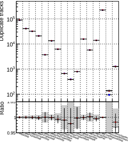
Number Configuration 1 DQM_V0001_R0000000001_Global_mkFit_jcore50maxCand-24DUPremoval-1000 2 DQM_V0001_R0000000001_Global_mkFit_jcore10maxCand-24DUPremoval-1000
