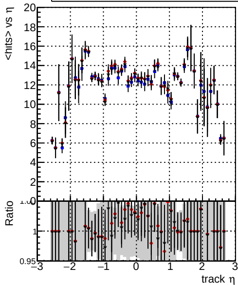
mean hits vs \eta Legend: DQM_V0001_R0000000001_Global_mkFit_baseline (blue), DQM_V0001_R0000000001_Global_mkFit_core50maxCand-24DUPremoval-1000 (red), DQM_V0001_R0000000001_Global_mkFit_core10maxCand-24DUPremoval-1000 (black)
