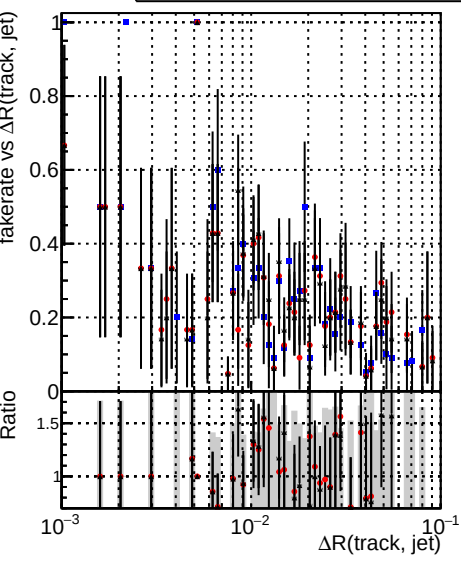
Fake rate vs \Delta R(\text{track, jet}) DQM_V0001_R000000001 Global mkFit baseline DQM_V0001_R000000001 Global mkFit_jcore50maxCand-24DUPremoval-1000 DQM_V0001_R000000001 Global mkFit_jcore10maxCand-24DUPremoval-1000
