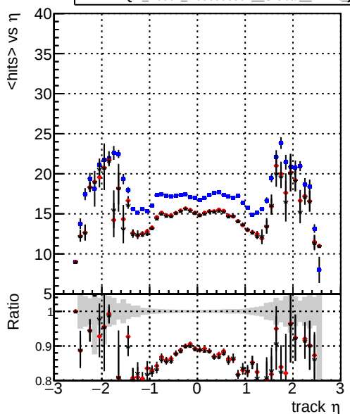
mean hits vs \eta — DQM_V0001_R000000001_Global_mkFit_baseline — DQM_V0001_R000000001_Global_mkFit_core50maxCand-24DUPremoval-1000 — DQM_V0001_R000000001_Global_mkFit_core10maxCand-24DUPremoval-1000
