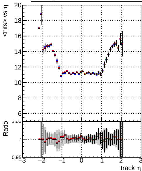
mean hits vs \eta DQM_V0001_R0000000001_Global_mkFit_baseline DQM_V0001_R0000000001_Global_mkFit_core50maxCand-24DUPremoval-1000 DQM_V0001_R0000000001_Global_mkFit_core10maxCand-24DUPremoval-1000
