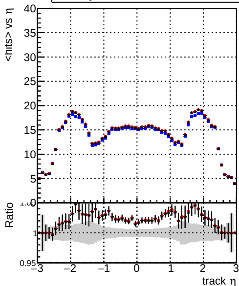
mean hits DQM_V0001_R0000000001_Global_mkFit_baseline DQM_V0001_R0000000001_Global_mkFit_core50maxCand-24DUPremoval-1000 DQM_V0001_R0000000001_Global_mkFit_core10maxCand-24DUPremoval-1000
