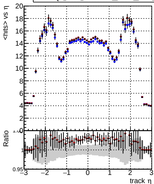
mean hits vs \eta Legend: - DQM_V0001_R0000000001_Global_mkFit_baseline (blue line) - DQM_V0001_R0000000001_Global_mkFit_core50maxCand-24DUPremoval-1000 (red line) - DQM_V0001_R0000000001_Global_mkFit_core10maxCand-24DUPremoval-1000 (black line)
