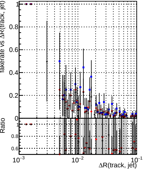
Fake rate vs \Delta R(\text{track, jet}) Legend: DQM_V0001_R000000001 Global mkFit baseline (blue dots) DQM_V0001_R000000001 Global mkFit_jcore50maxCand-24DUPremoval-1000 (red dots) DQM_V0001_R000000001 Global mkFit_jcore10maxCand-24DUPremoval-1000 (black dots)
