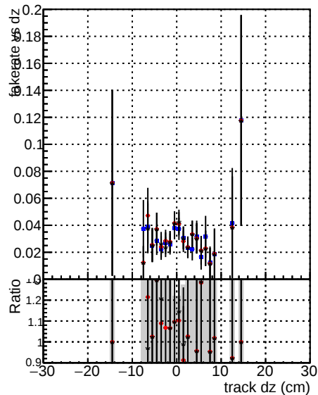
Legend for Fake rate vs d, Duplicates rate vs Dxy, and Pileup rate vs dxy plots: DOM V0001 R0000000001 Global mkFit baseline DOM V0001 R0000000001 Global mkFit [core10maxCand-24DUPremoval-1000]
