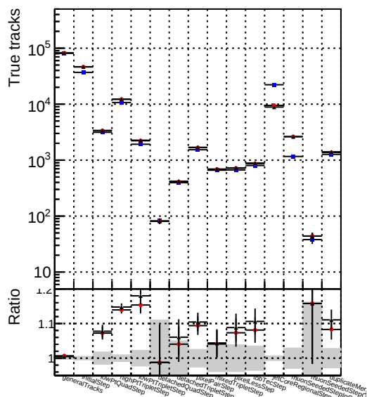
—●— DQM_V0001_R0000000001_Global_mkFit_baseline —●— DQM_V0001_R0000000001_Global_mkFit_jcore50maxCand-24DUPremoval-1000 —●— DQM_V0001_R0000000001_Global_mkFit_jcore10maxCand-24DUPremoval-1000
