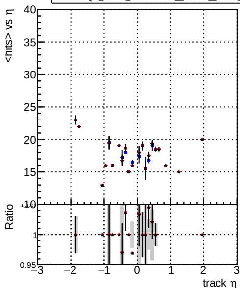
mean hits — DQM_V0001_R000000001_Global_mkFit_baseline — DQM_V0001_R000000001_Global_mkFit_core50maxCand-24DUPremoval-1000 — DQM_V0001_R000000001_Global_mkFit_core10maxCand-24DUPremoval-1000
