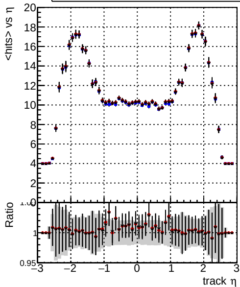
mean hits vs \eta — DQM_V0001_R0000000001_Global_mkFit_baseline — DQM_V0001_R0000000001_Global_mkFit_core50maxCand-24DUPremoval-1000 — DQM_V0001_R0000000001_Global_mkFit_core10maxCand-24DUPremoval-1000
