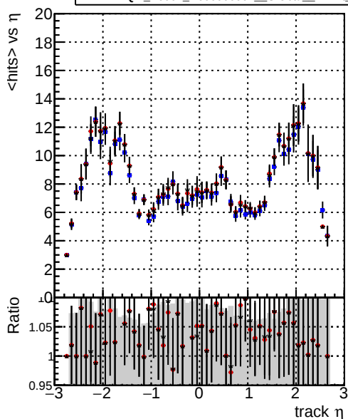
mean hit DQM_V0001_R000000001_Global_mkFit_baseline DQM_V0001_R000000001_Global_mkFit_core50maxCand-24DUPremoval-1000 DQM_V0001_R000000001_Global_mkFit_core10maxCand-24DUPremoval-1000
