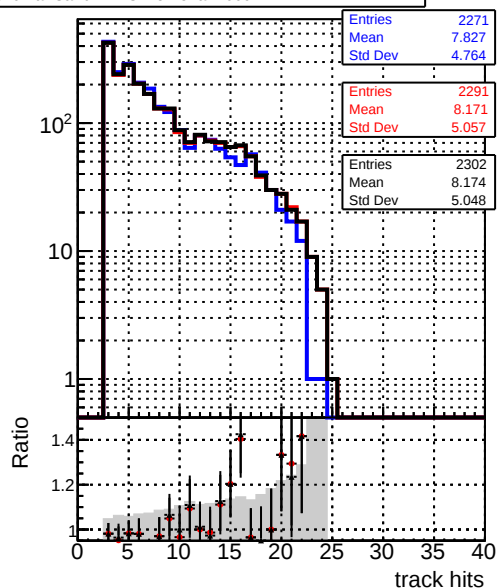
mean hit DQM_V0001_R000000001_Global_mkFit_baseline DQM_V0001_R000000001_Global_mkFit_core50maxCand-24DUPremoval-1000 DQM_V0001_R000000001_Global_mkFit_core10maxCand-24DUPremoval-1000
