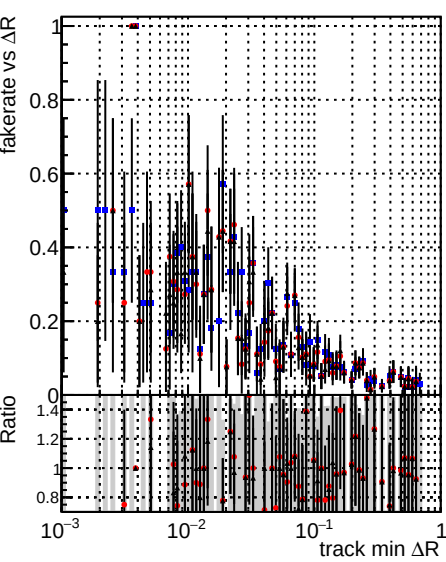
Fake rate vs \Delta R (track, jet) DQM V0001 R000000001 Global mkFit baseline DQM V0001 R000000001 Global mkFit jcore50maxCand-24DUPremoval-1000 DQM V0001 R000000001 Global mkFit jcore10maxCand-24DUPremoval-1000
