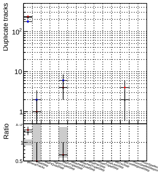
Number of tracks vs collection DQM_V0001_R0000000001_Global_mkFit_baseline DQM_V0001_R0000000001_Global_mkFit_core50maxCand-24DUPremoval-1000 DQM_V0001_R0000000001_Global_mkFit_core10maxCand-24DUPremoval-1000
