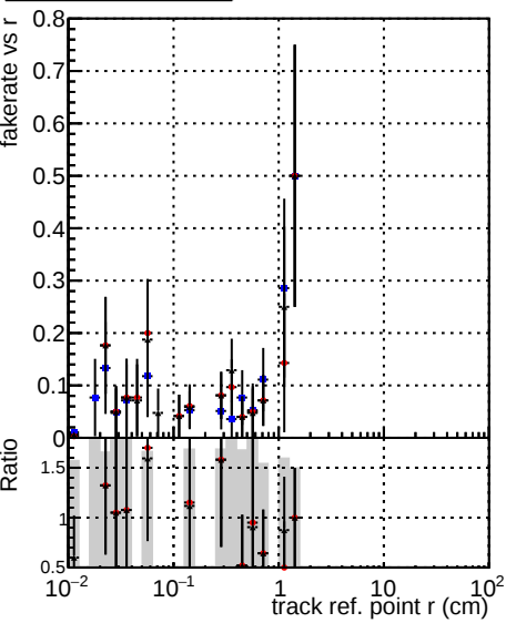
DQM_V0001_R0000000001 Global mkFit baseline DQM_V0001_R0000000001 Global mkFit jcore50maxCand-24DUPremoval-1000 DQM_V0001_R0000000001 Global mkFit jcore10maxCand-24DUPremoval-1000
