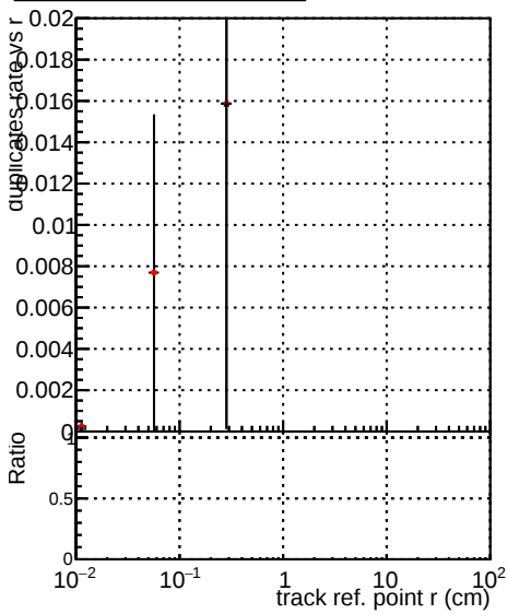
—●— DQM_V0001_R000000001 Global mkFit_baseline —●— DQM_V0001_R000000001 Global mkFit_jcore50maxCand-24DUPremoval-1000 —●— DQM_V0001_R000000001 Global mkFit_jcore10maxCand-24DUPremoval-1000
