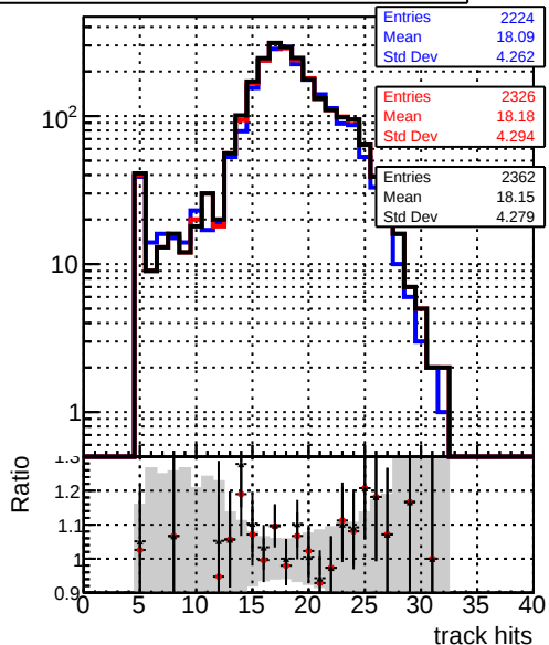
mean hits DQM_V0001_R0000000001_Global_mkFit_baseline DQM_V0001_R0000000001_Global_mkFit_core50maxCand-24DUPremoval-1000 DQM_V0001_R0000000001_Global_mkFit_core10maxCand-24DUPremoval-1000
